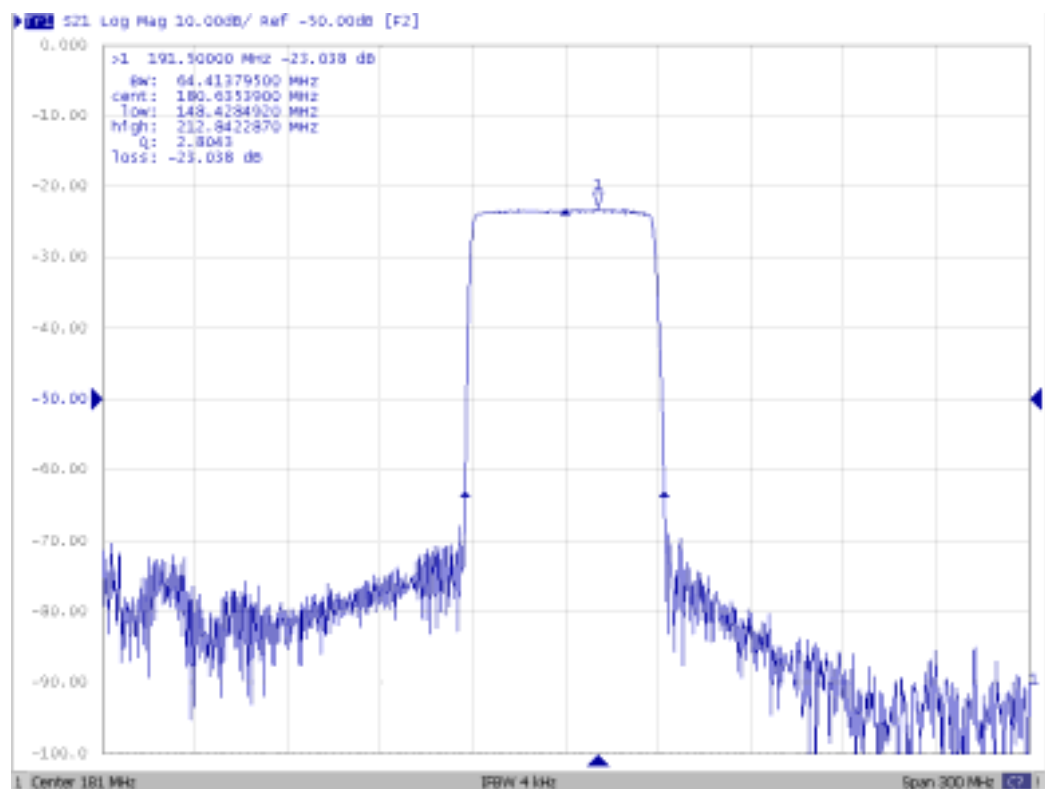
Fig1. Horizontal: 30MHz/Div Vertical: 10dB/Div
