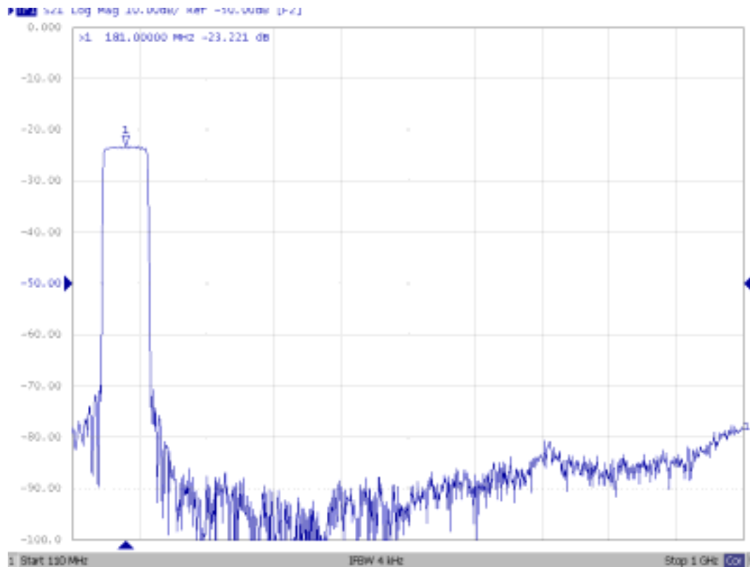
Fig1. Horizontal: 100MHz/Div Vertical: 10dB/Div
